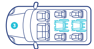
3. Conversion with fixed/removable second row seats and tip & turn third row seats (2 small wheelchairs in line)
